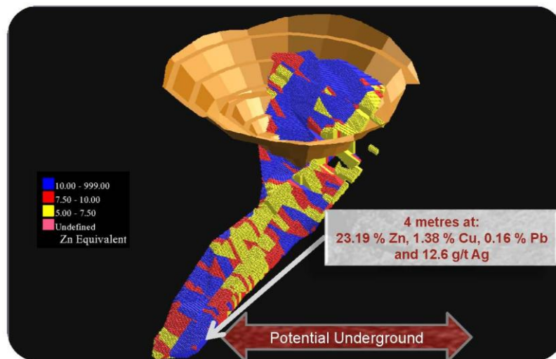
Figure 1 John Fardy Preliminary Mine Design
